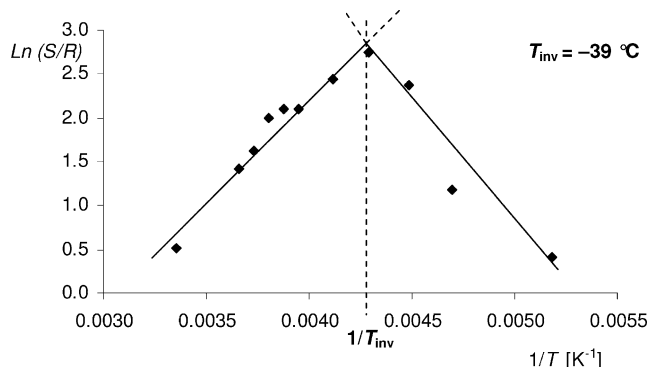
Figure 1. Eyring plot for the aza-Michael addition of p -anisidine ( 2a ) to N -acyloxazolidinone ( 1a ) catalyzed by samarium complex 5 .
