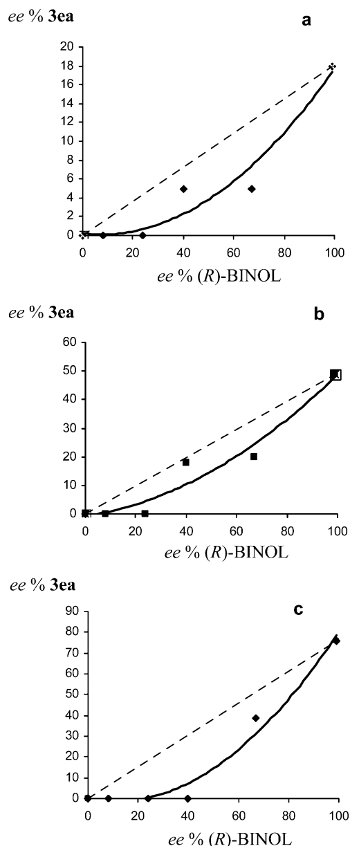
Figure 3. Correlation between the enantiomeric excess of binaphthol and the enantiomeric excess of aza-Michael adduct 3ea at a) 20, b) 0 and c) -40^{\circ}\text{C} .
