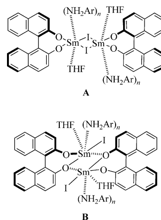
Scheme 3. Proposed dimeric structures for the catalytic species in the aza-Michael reactions.
