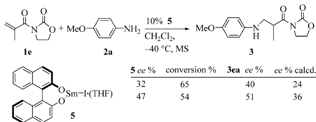
Scheme 2. Aza-Michael reaction catalyzed by mixtures of (R)- and (S)- 5 .
