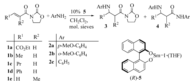
Scheme 1. Aza-Michael reaction of aromatic amines with N -alkenoyloxazolidinones catalyzed by iodido(binaphtholato)samarium.
