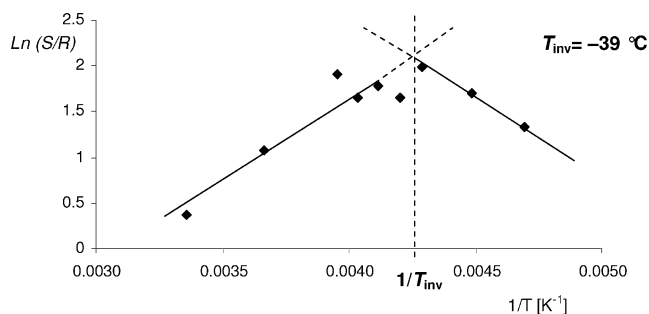
Figure 2. Eyring plot for the aza-Michael addition of p -anisidine ( 2a ) to N -acyloxazolidinone ( 1e ) catalyzed by samarium complex 5 .
